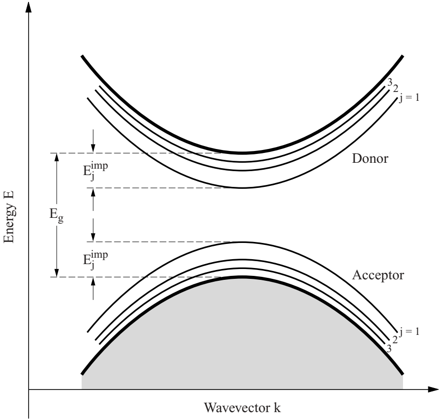
Fig. 6.13. Energy levels \mathcal{E}_j^{imp} of impurity states in the vicinity of the valence and conduction bands. Donors lead to energy levels below the bottom of the conduction band; the impurity levels of acceptors are above the valence band.
