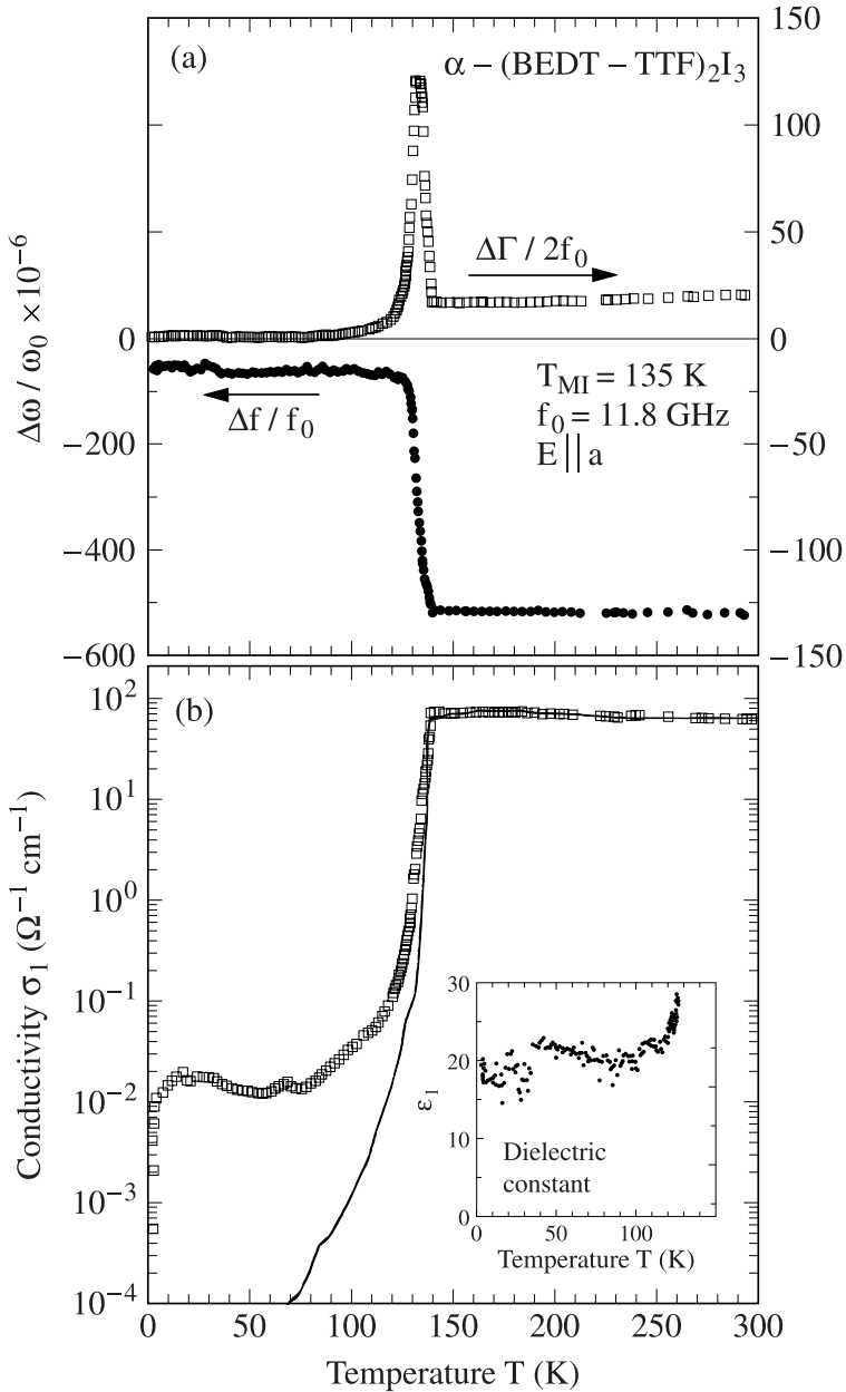
Fig. 11.15. (a) Temperature dependence of \Delta\Gamma/2f_0 and \Delta f/f_0 obtained on a sample of \alpha - (\text{BEDT} - \text{TTF})_2\text{I}_3 in an 11.8 GHz cavity. Near the phase transition, T_{\text{MI}}=135 K, a large change in the frequency shift \Delta f/f_0 occurs together with a peak in the bandwidth \Delta\Gamma/2f_0 . (b) The a axis conductivity observed in the microwave range is displayed together with the dc conductivity. Below the metal–insulator phase transition, the high frequency conductivity develops a plateau while the dc values continue to decrease. The temperature dependence of the dielectric constant is displayed in the inset (after [Dre93]).
