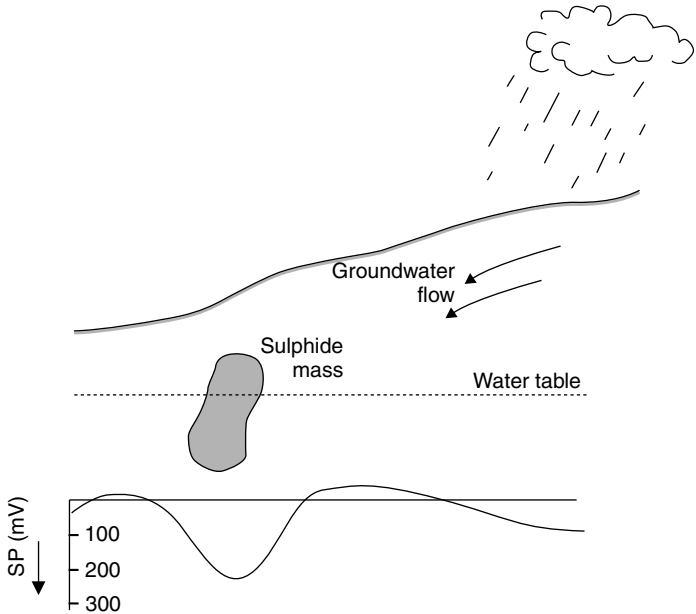
Figure 7.1 Sources of SP effects. The sulphide mass straddling the water table concentrates the flow of oxidation–reduction currents, producing a negative anomaly at the surface. The downslope flow of groundwater after rain produces a temporary SP, in this case inversely correlated with topography.
