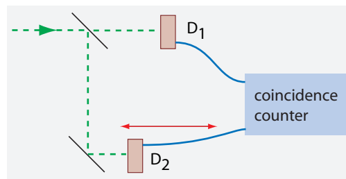
FIGURE 294 How to measure photon statistics: with an electronic coincidence counter and the variation by varying the geometrical position of a detector
