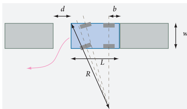
FIGURE 400 Leaving a parking space – the outer turning radius
