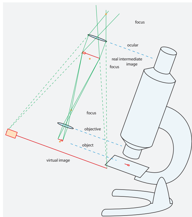
FIGURE 407 Two converging lenses make a microscope
