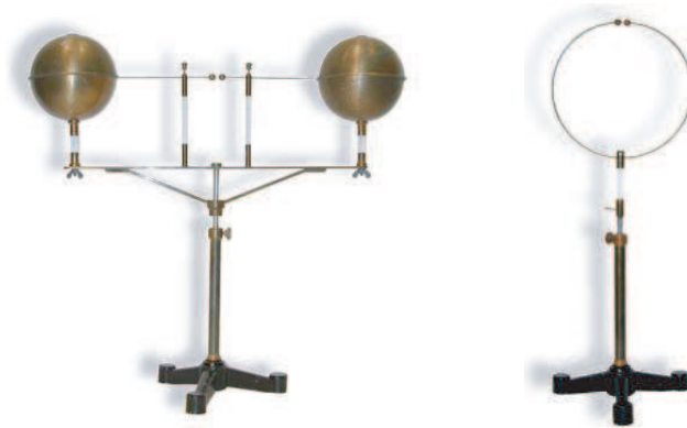
FIGURE 245 The first transmitter (left) and receiver (right) of electromagnetic (micro-) waves
