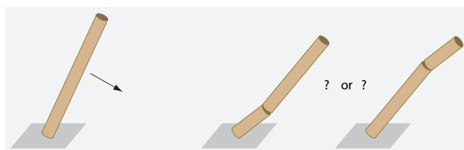
FIGURE 91 How and where does a falling brick chimney break?
