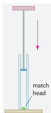
FIGURE 120 The fire pump
