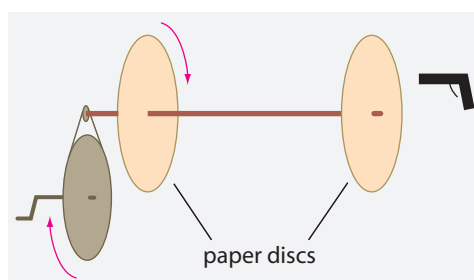
FIGURE 399 A simple way to measure bullet speeds
