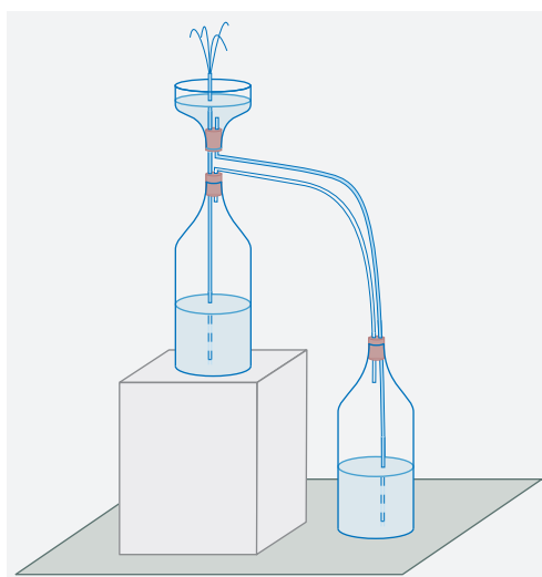
FIGURE 115 Heron's fountain
