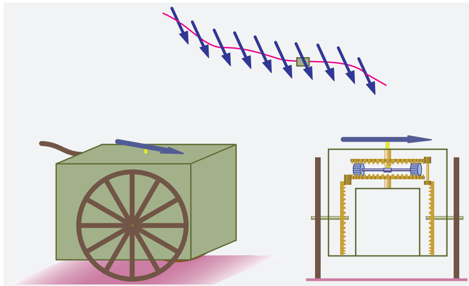
FIGURE 405 The south-pointing carriage
