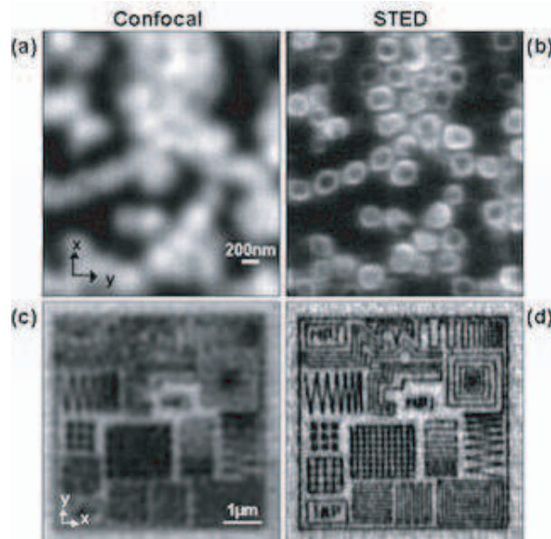
FIGURE 271 Sub-wavelength optical microscopy using stimulated emission depletion (© MPI für biophysikalische Chemie/Stefan Hell)
