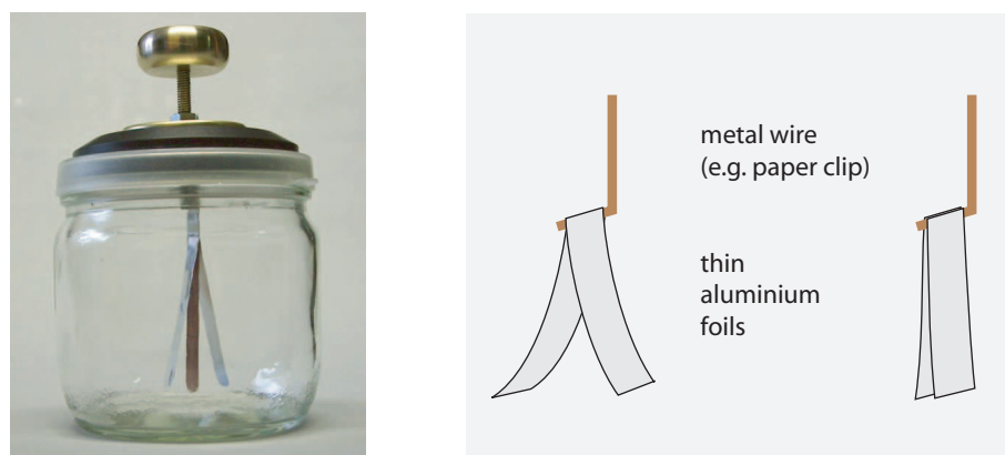
FIGURE 347 An electrostatic demonstrator (© Harald Chmela) and its charged (left) and uncharged state (right)
