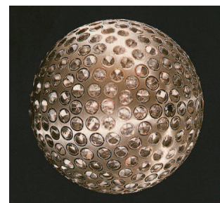
FIGURE 183 The LAGEOS satellites: metal spheres with a diameter of 60 cm, a mass of 407 kg, and covered with 426 retroreflectors
