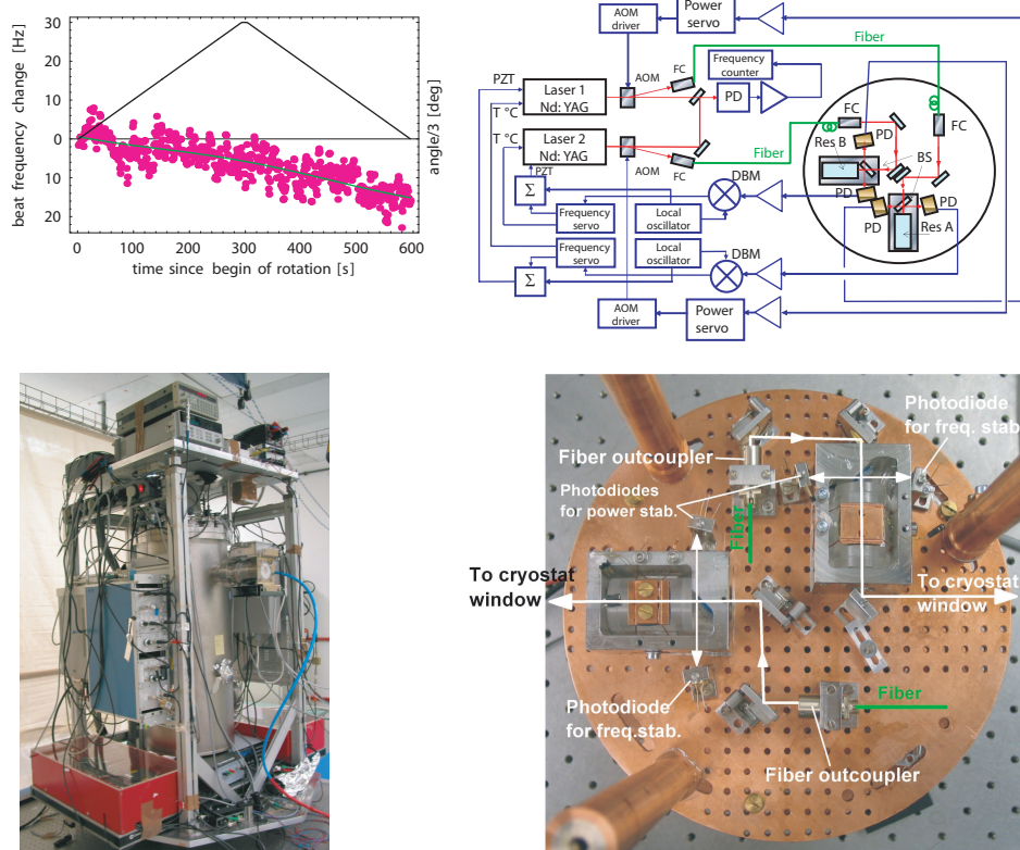
FIGURE 143 The result, the schematics and the cryostat set-up for the most precise Michelson–Morley experiment performed to date (© Stephan Schiller)
