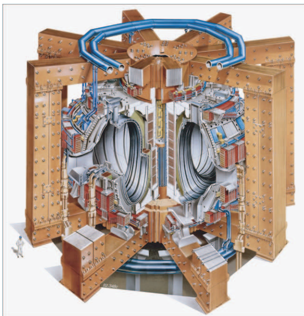
FIGURE 354 A simplified drawing of the Joint European Torus in operation at Culham, showing the large toroidal chamber and the magnets for the plasma confinement (© EFDA-JET)
