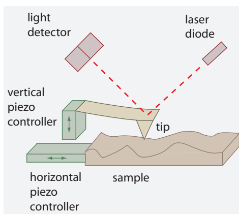
FIGURE 111 The principle, and a simple realization, of an atomic force microscope
