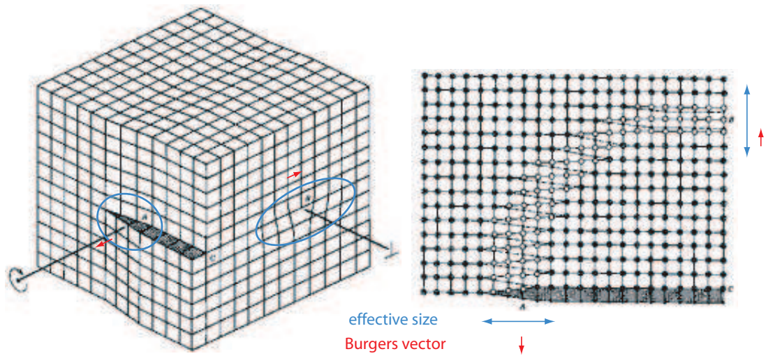
FIGURE 376 The two pure dislocation types: edge and screw dislocations
