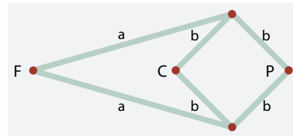
FIGURE 89 How to draw a straight line with a compass: fix point F, put a pencil into joint P and move C with a compass along a circle
